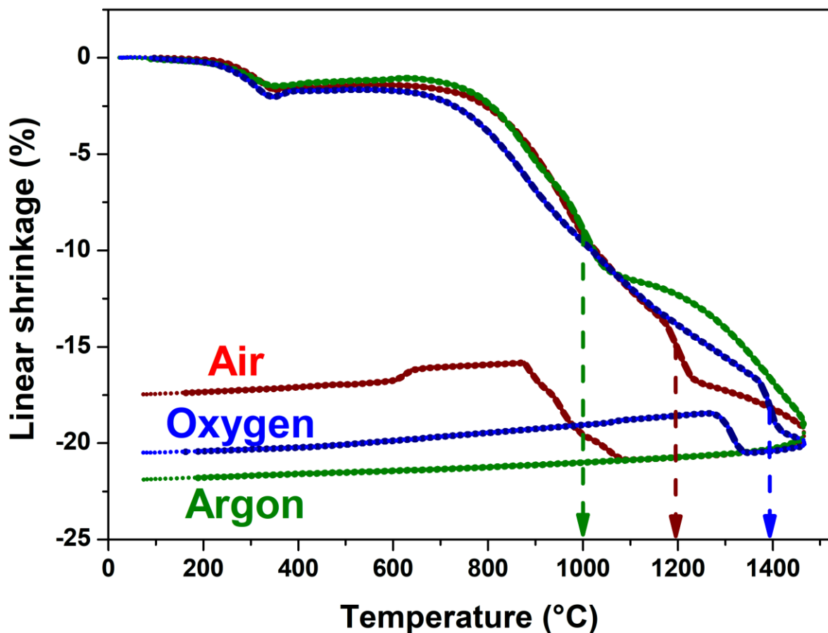
Figure 2. Linear shrinkage of \text{Pr}_6\text{O}_{11} green pellets heat-treated under argon, air or oxygen as a function of temperature ( 5^\circ\text{C}/\text{min} heating and cooling rates).
