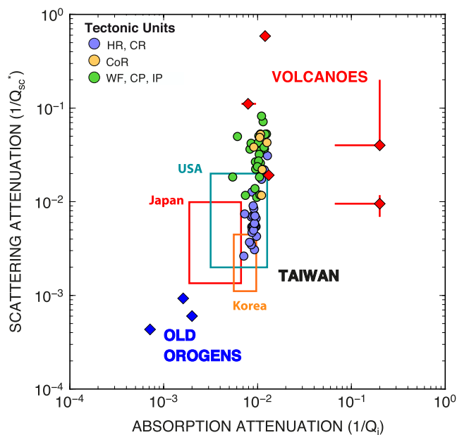
Figure 11. Q_{sc}^{-1} and Q_i^{-1} in the frequency band 1–2 Hz for Taiwan (circles) and other regions of the world (diamonds and boxes). Colored circles indicate similar tectonic units in Taiwan: crystalline massifs (HR and CR) are in blue, sedimentary and highly tectonized areas (Western Foothills, Coastal Plain, and Ilan Plain) are in green, and stations in Coastal Range and Longitudinal Valley (volcanic materials) are in yellow. Old orogens (mainly western Europe) are marked by blue diamonds (Lacombe et al., 2003; Sens-Schönfelder & Wegler, 2006; Sens-Schönfelder et al., 2009) and volcanoes by red diamonds (Del Pezzo et al., 2001; Mayeda et al., 1992; Ugalde et al., 2010; Wegler, 2003). Minimum and maximum values for absorption and scattering in Japan (Carcolé & Sato, 2010), Korea (Rachman et al., 2015) and North America (Eulenfeld & Wegler, 2017) are also shown.
