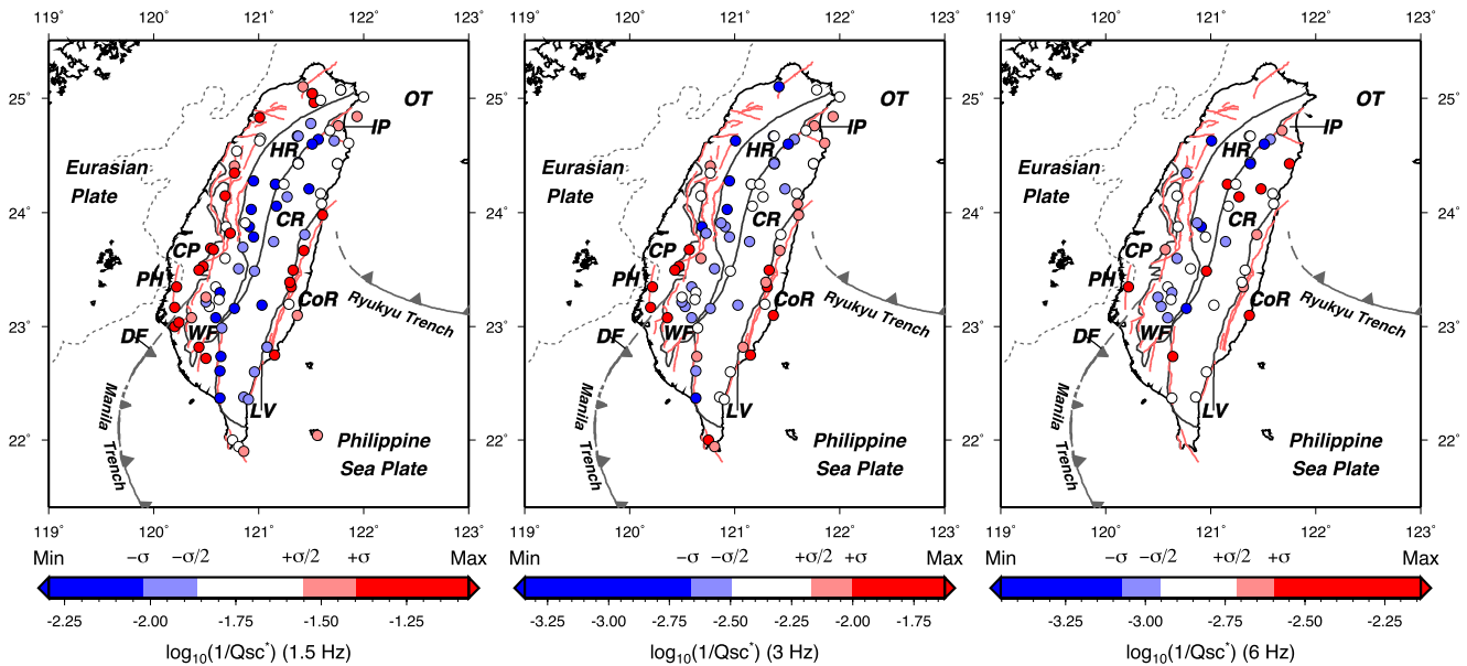
Figure 7. Total scattering maps ( 1/Q_{sc}^* ) in three frequency bands: results of multiple lapse time window analysis are plotted at the location of the station. Values higher (resp. lower) than the average one are shown in red (resp. blue). The scale indicates the maximum and the minimum values in each frequency band. Pink lines are surface traces of active faults from Shyu et al. (2016) and the five major lithotectonic units are delineated with thick dark lines (see Figure 1 for more details).
