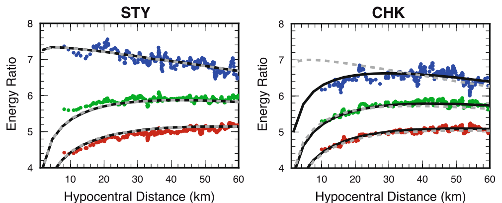
Figure 3. Fit of multiple lapse time window analysis measurements (dots) at stations STY (left) and CHK (right) using isotropic (dashed line) or anisotropic scattering models (solid line). Scattering anisotropy (backscattering) clearly improves the agreement with data at station CHK.
