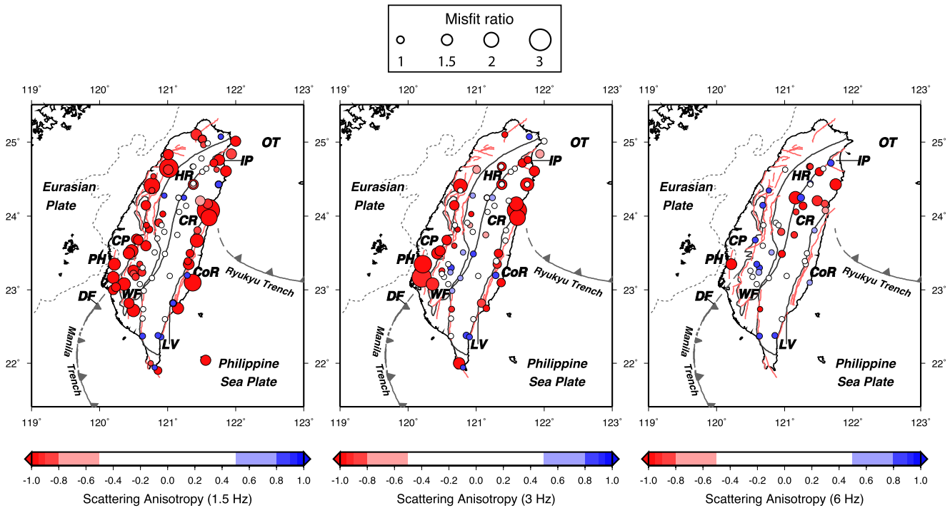
Figure 10. Scattering anisotropy ( g ) maps in three frequency bands: results of multiple lapse time window analysis are plotted at the location of the station. Models with strong backscattering (resp. strong forward scattering) are shown in red (resp. blue). Isotropic models are in white. The size of the circles correspond to the misfit ratio between isotropic and anisotropic models ( \chi_{iso}^2/\chi_{aniso}^2 ). Pink lines are surface traces of active faults from Shyu et al. (2016) and the five major lithotectonic units are delineated with thick dark lines (see Figure 1 for more details).
