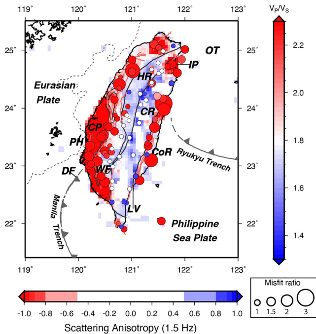
Figure 13. Comparison between the scattering anisotropy g at 1.5 Hz (colored circles) and the velocity ratio V_P/V_S at the surface (background color on the right) (Huang et al., 2014). Models with strong backscattering (resp. strong forward scattering) are shown in red (resp. blue). Isotropic models are in white. The size of the circles correspond to the misfit ratio between isotropic and anisotropic models ( \chi_{\text{iso}}/\chi_{\text{anis}} ). Pink lines are surface traces of active faults from Shyu et al. (2016) and the five major lithotectonic units are delineated with thick dark lines (see Figure 1 for more details).
