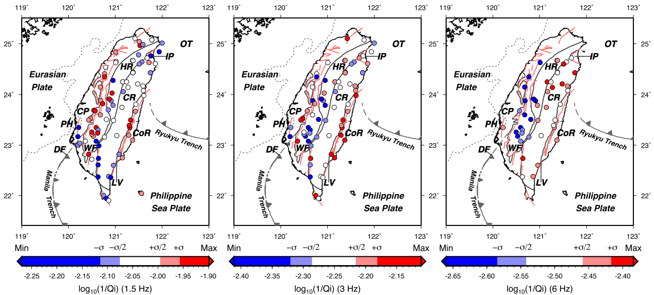
Figure 8. Absorption maps ( 1/Q_i ) in three frequency bands: results of multiple lapse time window analysis are plotted at the location of the station. Values higher (resp. smaller) than the average one are shown in red (resp. blue). The scales indicate the maximum and the minimum values in each frequency band. Pink lines are surface traces of active faults from Shyu et al. (2016) and the five major lithotectonic units are delineated with thick dark lines (see Figure 1 for more details).
