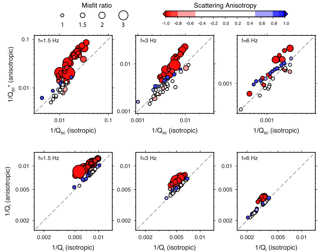
Figure 6. Comparison of scattering and intrinsic attenuation ( 1/Q_{sc}^* and 1/Q_i ) between isotropic and anisotropic models in three frequency bands [1–2], [2–4], [4–8] Hz. The scattering anisotropy g is given by the color scale (negative values are in red and positive ones in blue). The size of the circles indicates the misfit ratio between isotropic and anisotropic models ( \chi_{iso}^2/\chi_{aniso}^2 ).
