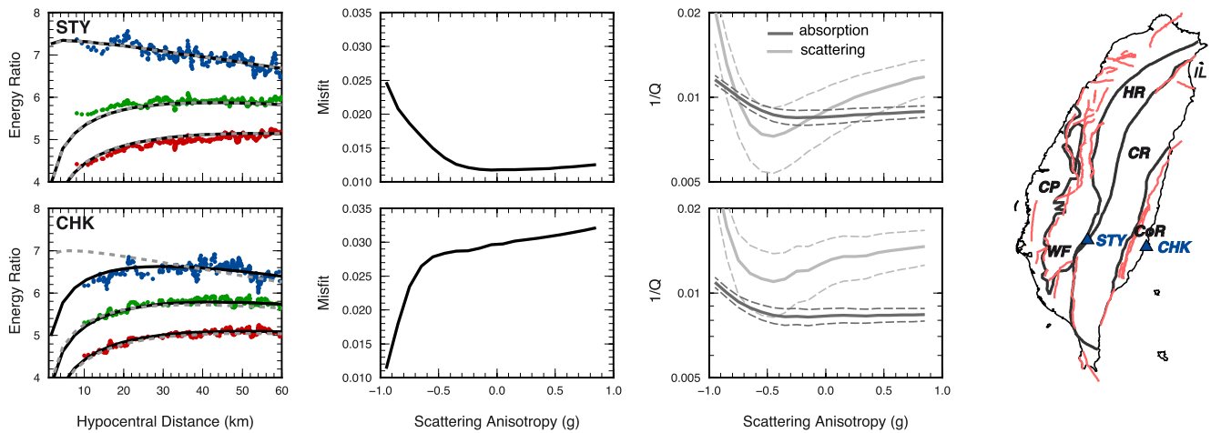
Figure 5. Illustrations of multiple lapse time window analysis measurements and inversion results in the frequency band [1–2] Hz for two example stations, STY and CHK. Results for other stations are shown in Figures S2 to S14 in Supporting Information S1. Energy ratio measurements (dots), the best-fitting isotropic (dashed lines) and anisotropic (solid lines) models are shown on the left panels, where blue, green and red dots correspond to energy ratios in the first, second and third window, respectively. The station locations are indicated on the map furthest to the right: red lines are surface traces of active faults from Shyu et al. (2016) and the five major lithotectonic units are delineated with thick dark lines. The middle panels show the misfit as a function of the scattering anisotropy ( g ), while the right panels indicate 1/Q_i (black solid lines) and 1/Q_{sc}^* (gray solid lines) for the best models as a function of the scattering anisotropy ( g ) with standard errors delineated by dashed lines.
