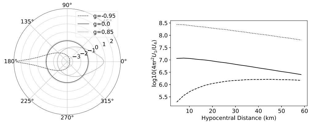
Figure 4. Effect of scattering anisotropy on the spatial distribution of energy contained in the early coda. The polar plot shows the scattering patterns for different values of the anisotropy parameter g , as indicated in inset, and the corresponding normalized energy ratios are shown on the right. Note that a logarithmic scale is used for the polar plot.
