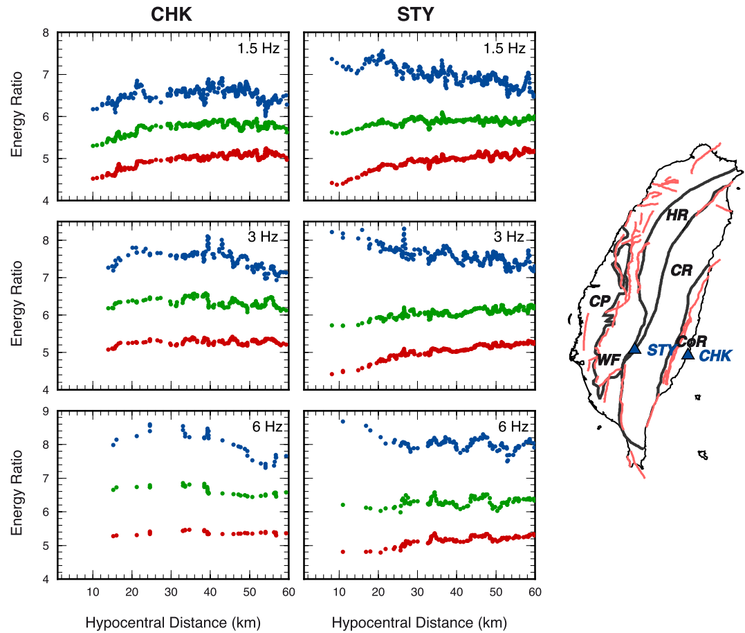
Figure 2. Examples of multiple lapse time window analysis measurements in three frequency bands [1–2], [2–4], and [4–8] Hz (from top to bottom) at two stations (CHK, STY) located in two distinct tectonic regions of Taiwan (map). Examples of records and envelopes are shown in Figure S1 in Supporting Information S1. Blue, green and red dots correspond to the logarithm of the energy ratio in the first, second and third window, respectively, corrected for the geometrical spreading 4\pi r^2 , where r is the hypocentral distance. In the map, surface traces of active faults from Shyu et al. (2016) are shown in red lines and the major lithotectonic units are delineated with thick dark lines.
