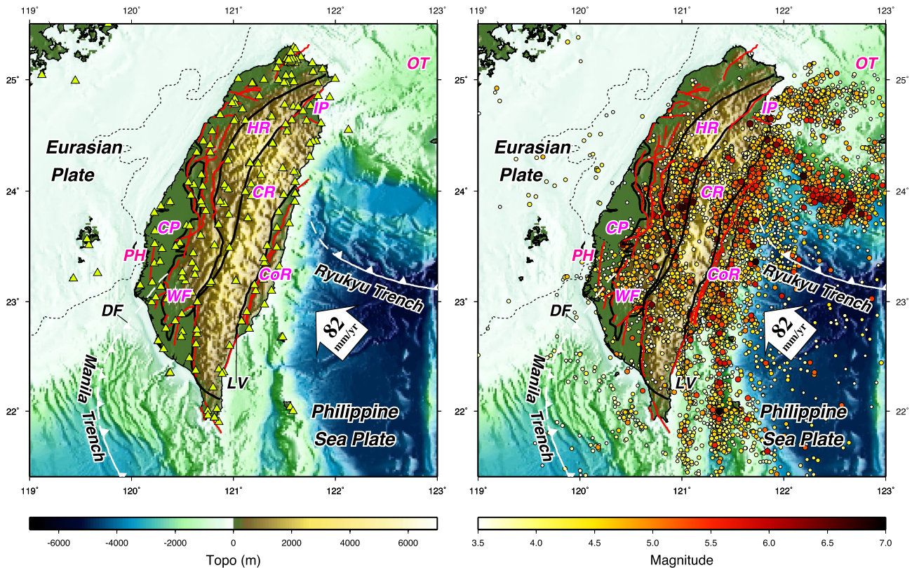
Figure 1. Topographic and tectonic map of Taiwan which mainly results from the oblique convergence between the Philippine Sea Plate (PSP) and the Eurasian Plate (EP). The white arrow indicates the velocity vector of the PSP relative to the EP. The boundaries of plate convergence along the Manila Trench in the south and the Ryukyu Trench in the northeast of Taiwan are shown in white with arrowheads indicating opposite subduction polarities. The dashed line indicates a 2000-m isopach of the Cenozoic sediments from A. Lin et al. (2003). Surface traces of active faults from Shyu et al. (2016) are shown in red lines. The geology of Taiwan is characterized by five major lithotectonic units (delineated with thick dark lines): from west to east, the Coastal Plain (CP), the Western Foothills (WF), the Hsuehsan Range (HR), the Central Range (CR), and the Coastal Range (CoR). The deformation front (DF), also the boundary between the CP and WF denoted by a dashed white line, extending northward from the northern Manila trench offshore SW Taiwan to the northern coast of Taiwan marks the frontal limit of collision-related deformation. The longitudinal Valley (LV) corresponds to the collision suture zone between the EP and PSP. The Okinawa Trough (OT) behind the Ryukyu arc-trench system is a back-arc rifting basin which migrates southwestward to the Ilan Plain (IP) in northeast Taiwan. The map also shows the seismological stations used in the present study (left panel) and the distribution of earthquakes (right panel) which occurred between 1994 and 2016 with a focal depth shallower than 40 km and a local magnitude greater than 3.5 reported from the Central Weather Bureau of Taiwan.
