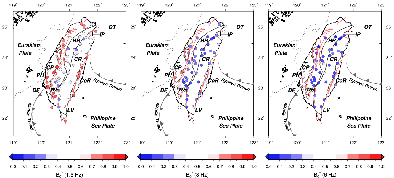
Figure 9. Albedo maps ( B_0^* = Q_{sc}^{-1} / (Q_i^{-1} + Q_{sc}^{-1}) ) in three frequency bands: results of multiple lapse time window analysis are plotted at the location of the station. Red (resp. blue) colors indicate that scattering (resp. absorption) dominates over absorption. Pink lines are surface traces of active faults from Shyu et al. (2016) and the five major lithotectonic units are delineated with thick dark lines (see Figure 1 for more details).
