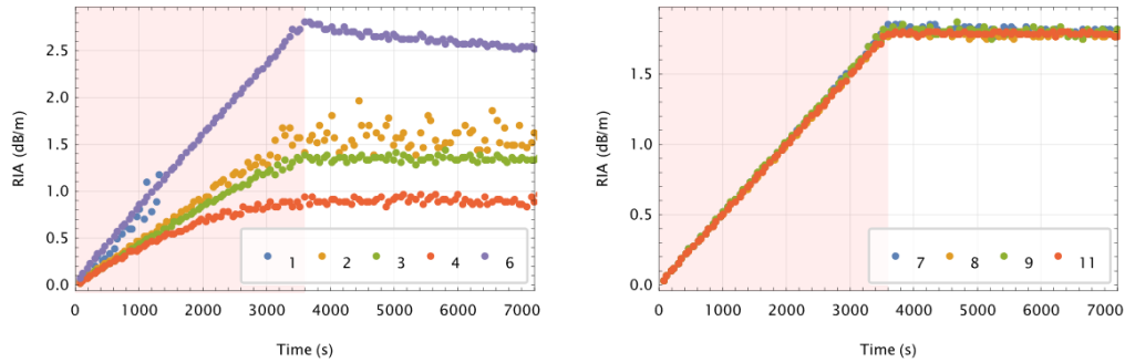
Fig. 5. RIA vs. time for Al-doped (left) and Al/Tm co-doped fibers (right) at wavelengths of high sensitivity, respectively 575 nm and 490 nm. The pink background part corresponds to irradiation, and the white one to fading. Only 1 Gy/h irradiations are shown here.
