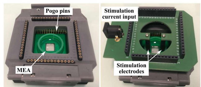
FIGURE 2. Left: Photograph of the custom MEA holder, which contacts the MEA pads through pogo-pins (spring-loaded contacts). Right: Photograph of the MEA holder topped with the stimulation PCB. Stimulation current is flowing between the two carbon electrodes.
