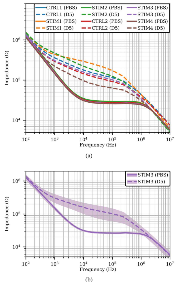
FIGURE 6. (a) Impedance spectroscopy before cell seeding with PBS (line) and after 5 days of differentiation (dashed line) on the 6 MEAs, mean values for 10-15 electrodes pairs. (b) One MEA (STIM3), all 15 measured electrodes, mean value ± standard deviation. PBS = only PBS on the MEA; D5 = myotubes on MEA at 5 th day of differentiation.
