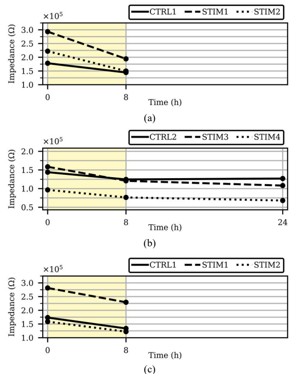
FIGURE 8. Mean bioimpedance at 10 kHz over time during day for CTRL1, STIM1-2 (a), and for CTRL2, STIM3-4 (b), and during day 2 for CTRL1, STIM1-2 (c). The yellow areas indicate the stimulation periods (pattern 1).
