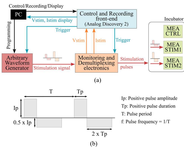
FIGURE 3. (a) Schematic of the stimulation system: the stimulation signal is generated by a programmable arbitrary waveform generator and delivered to 2 wells (MEAs) placed in an incubator. Signals travels through an interface allowing the demultiplexing of the pulses. A multifunction instrument ( Analog Discovery 2 ) controls this interface and performs the acquisition of the stimulation current and voltage. A computer controls this instrument and the generator. (b) Parameters of a stimulation waveform composed of asymmetric biphasic pulses: I_p and T_p are the amplitude and duration of the positive pulse respectively, T is the pulse period and f is the pulse frequency. Each positive pulse is balanced with a follow-up negative pulse (amplitude 0.5 \times I_p , duration 2 \times T_p ) delivering the same quantity of opposite charge.
