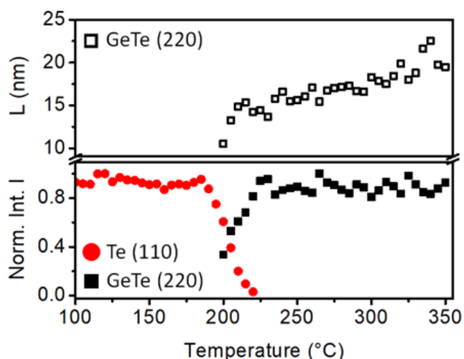
Fig. 2 Normalized integrated intensities of diffraction peaks and average grain size ( L ) during in situ XRD isochronal annealing of \sim 0.9 ^{\circ}\text{C min}^{-1} of Te-on-Ge bilayer: hex-Te (110) (red circles) and \alpha -GeTe (220) (black squares).
