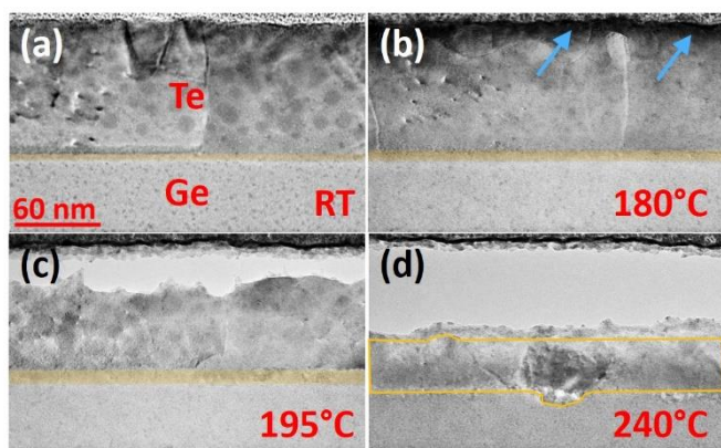
Fig. 5 Cross-section TEM images acquired during in situ heating of a Te-on-Ge bilayer from RT to 240 °C: a) RT; b) 180 °C, the blue arrows indicate the voids formation; c) 195 °C; d) 240 °C. The added color highlights the new phase.
