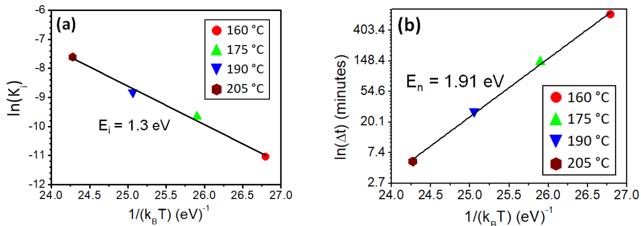
Fig. 4 (a) Variations of \ln(K) , with K , the interface reaction rate, as a function of the inverse of temperature for \alpha -GeTe growth during the Te-on-Ge bilayer reactive diffusion; (b) Variations of the nucleation time \ln(\Delta t) as a function of the inverse of temperature for GeTe nucleation during Te-on-Ge bilayer reactive diffusion.
