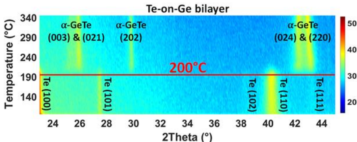
Fig. 1 XRD patterns ( \lambda = 0.154 nm) as a function of temperature acquired during in situ isochronal annealing of \sim 0.9 K \text{min}^{-1} for Te-on-Ge bilayer. The color plot panel is in counts/s.
