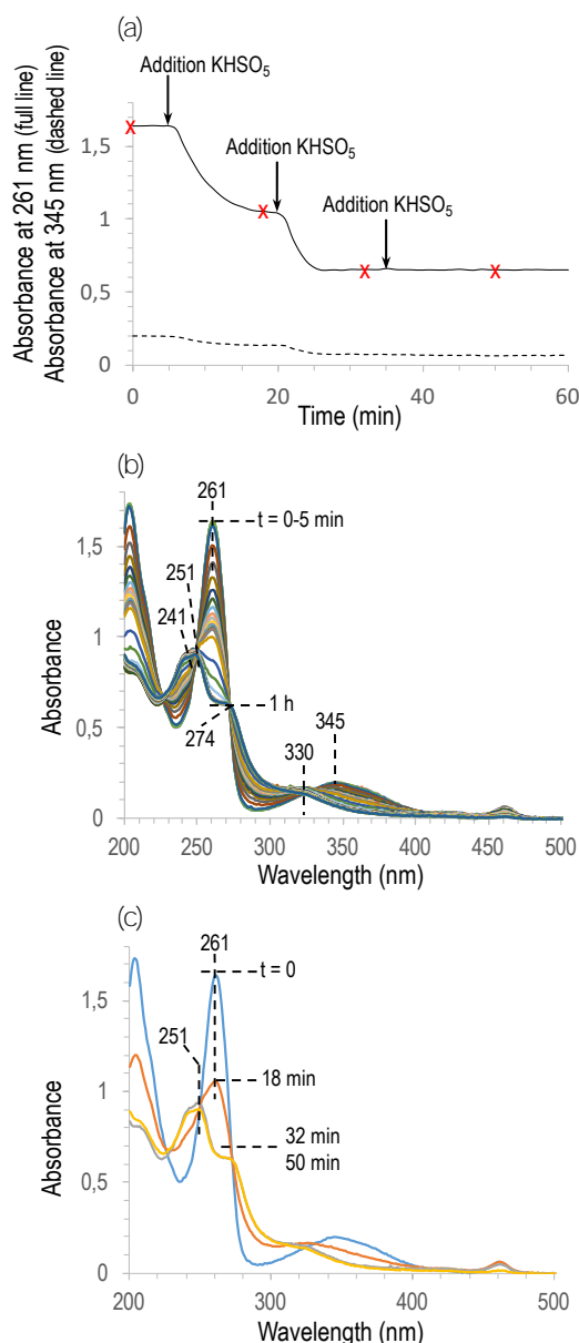
Figure 2. (a) Absorbance at 261 nm and 345 nm according to the reaction time upon three successive additions of \text{KHSO}_5 (2 mol equiv each) at 5 min, 20 min and 35 min; Spectra at t = 0 , 18 min, 32 min and 50 min (red crosses) are depicted in Figure 2c; (b) UV-visible kinetic spectra of the catalytic oxidation of TDMQ20 (50 \mu\text{M} ) by three successive additions of \text{KHSO}_5 2 mol equiv in the presence of MnTMPyP 1 mol% in \text{H}_2\text{O}/\text{CH}_3\text{CN} , 1/1, v/v; time interval between two successive spectra was 1 min; (c) Spectra at t = 0 (blue), 18 min (orange), 32 min (grey) and 50 min (yellow). Absorbance at 462 nm is due to MnTMPyP catalyst.
