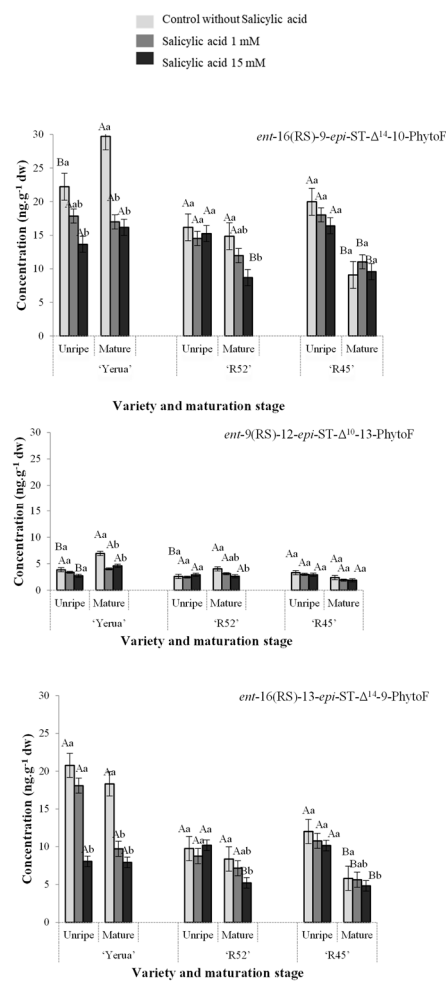
Figure 3. Comparison of concentrations of the individual phytofurans ent-16(RS)-9-epi-ST-Δ 14 -10-PhytoF , ent-9(RS)-12-epi-ST-Δ 10 -13-PhytoF and ent-16(RS)-13-epi-ST-Δ 14 -9-PhytoF in unripe and mature rice grains at different salicylic acid supplementation levels (untreated, 1 mM, and 15 mM) in each genotype ('Yerua', 'R52', and 'R45'). Distinct capital letters indicate significant differences between the maturation stage of rice grains at harvest for the same genotype, and different lowercase letters indicate significant differences between SA levels for the same genotype, both at p < 0.05 , according to one-way analysis of variance (ANOVA) and multiple range test of Tukey.
