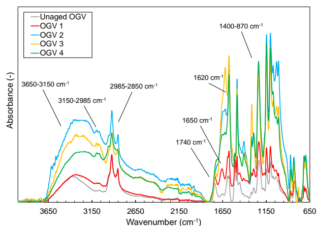
Figure 3. FTIR spectra of OGV surfaces (upper side).
