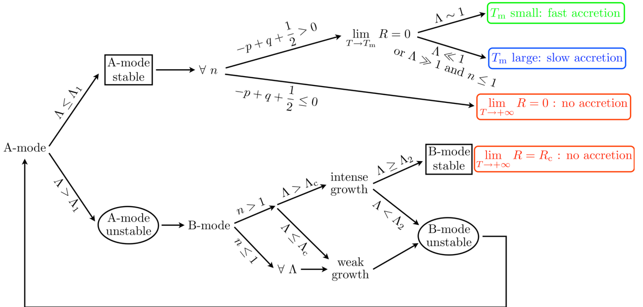
Figure 7. Summary of the global evolution of an initially small growing grain. For intense accelerating growth, particles decouple from the gas at a finite radius, staying in the B mode of migration. Otherwise, grains survive the radial-drift barrier if they pile-up, i.e. if -p + q + 1/2 \leq 0 since they migrate in the A mode. The grains radial migration is always more efficient when the ratio between growth and migration time-scales is of the order of unity.
