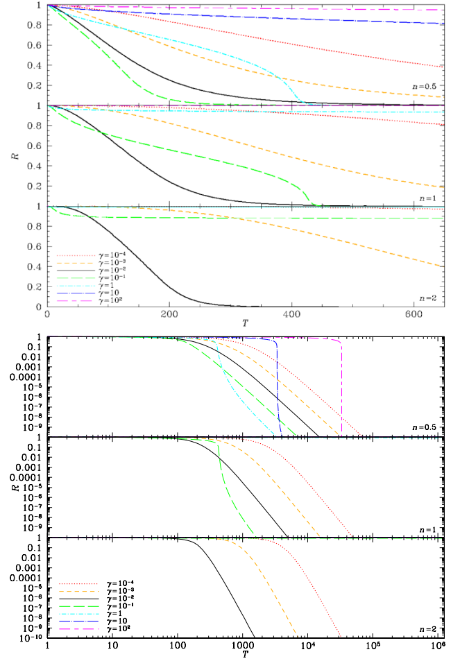
Figure B2. Same as Fig. B1 for p = 3/2 and q = 3/4 .
