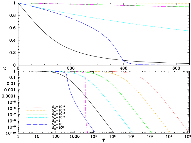
Figure 2. Same as Fig. 1 for p = 3/2 and q = 3/4 ( -p + q + \frac{1}{2} < 0 ). Grains experience a pile-up which prevents them from being accreted on to the central star. Compare the black curve of this figure with the black curve of Fig. 1 to clearly see the grain's pile-up.
