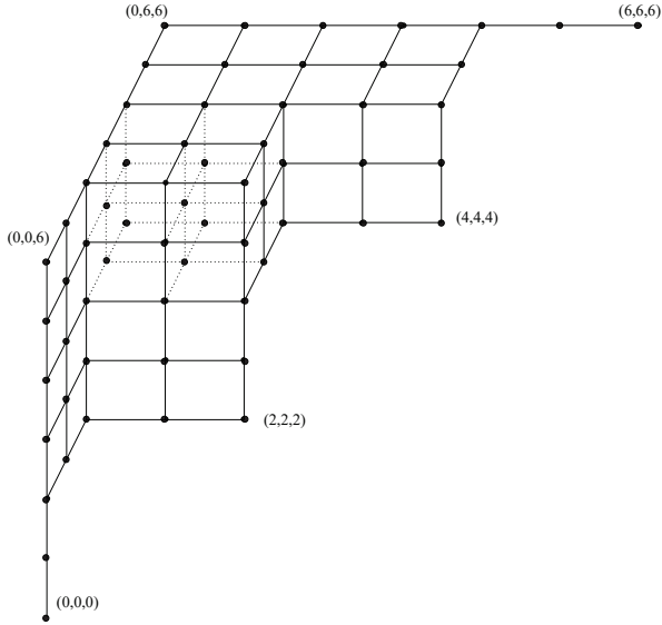
Figure 3. The lattice (\mathcal{P}, \leq) for p = 3 .
