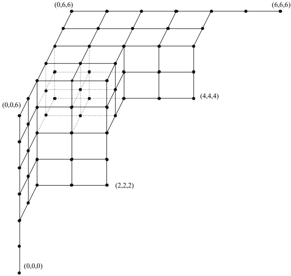
Figure 3. The lattice (\mathcal{P}, \preceq) for p = 3 .
