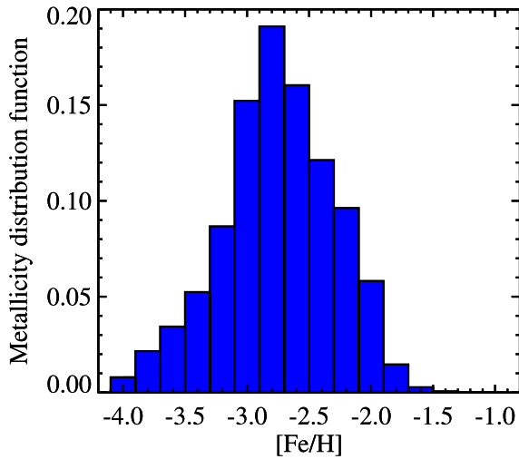
Figure 2. Metallicity distribution of Ret II, as determined from the spectroscopic metallicity measurements of Simon et al. (2015a). Each individual stellar metallicity is modeled as a Gaussian probability distribution, and samples are drawn from the combined probability distribution from all 16 stars.
