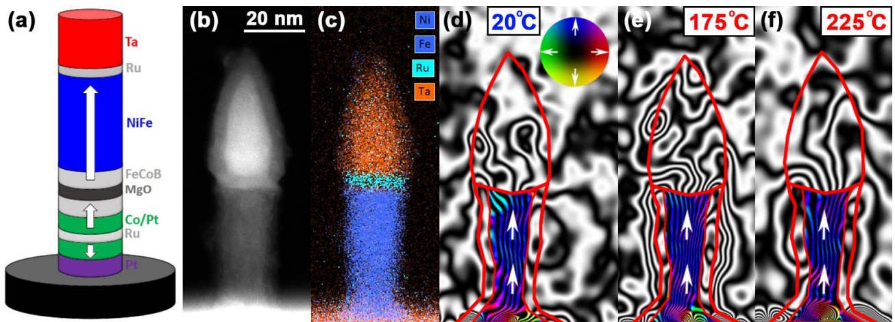
Figure 2. (a) Schematic of a PSA-STT-MRAM MTJ cell with a 60 nm NiFe storage layer, where the white arrows denote the expected magnetic easy axis 2 . (b) STEM image of a first PSA pillar with a diameter of ~ 20nm; and (c) the associated EDX chemical map showing the elemental distribution of Ta (red), Ni/Fe (blue) and Ru (turquoise). (d-f) Magnetic induction maps reconstructed from electron holograms acquired during in-situ heating at (d) 20°C; (e) 175°C; and (f) 225°C. The contour spacing is 0.042 rad for all the magnetic induction maps, and the magnetization direction is shown using white arrows, as depicted in the color wheel.
