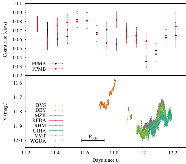
Figure 2. Top panel: the background-subtracted 3.0–30 keV NuSTAR light curve of V1674 Her (see Section 3.1.1). Bottom panel: simultaneous optical V band photometry by multiple observers identified by their AAVSO codes. The horizontal bar indicates the duration of V1674 Her orbital period.
