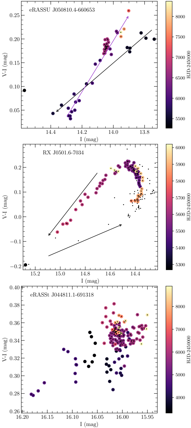
Fig. 8. OGLE V-I colour index as a function of I for eRASSU J050810.4–660653 ( top ), RX J0501.6–7034 ( middle ), and eRASSt J044811.1–691318 ( bottom ). The I values are interpolated to the times of the V -band observations. Due to the fast brightness changes seen from RX J0501.6–7034 the interpolated I values are only used when an I measurement exists within five days of the V -band observation.
