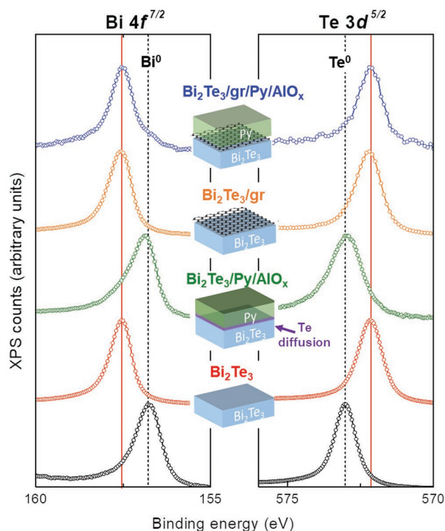
Figure 3. X-ray photoemission spectroscopy at the \text{Bi}4f^{7/2} and \text{Te}3d^{5/2} peaks for different stacks with and without graphene interlayer. From bottom to top: pure \text{Bi}^0 and \text{Te}^0 (black symbols), \text{Bi}_2\text{Te}_3 (red symbols), \text{Bi}_2\text{Te}_3 /graphene (orange symbols), \text{Bi}_2\text{Te}_3 /Py/ \text{AlO}_x (green symbols) and \text{Bi}_2\text{Te}_3 /graphene/Py/ \text{AlO}_x (blue symbols). The peak positions for pure \text{Bi}^0 and \text{Te}^0 (dotted black line), as well as those corresponding to \text{Bi}_2\text{Te}_3 (solid red line), are indicated as references. Data from samples not containing graphene was taken from reference [8].
