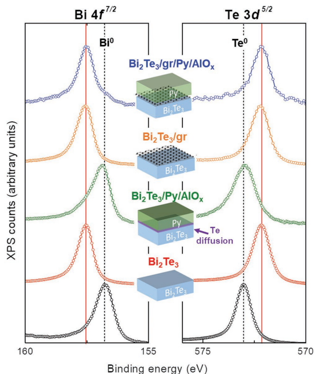
Figure 3. X-ray photoemission spectroscopy at the \text{Bi}4f^{7/2} and \text{Te}3d^{5/2} peaks for different stacks with and without graphene interlayer. From bottom to top: pure \text{Bi}^0 and \text{Te}^0 (black symbols), \text{Bi}_2\text{Te}_3 (red symbols), in situ grown \text{Bi}_2\text{Te}_3 /Py/ \text{AlO}_x (green symbols), \text{Bi}_2\text{Te}_3 /graphene (orange symbols) and \text{Bi}_2\text{Te}_3 /graphene/Py/ \text{AlO}_x (blue symbols). The peak positions for pure \text{Bi}^0 and \text{Te}^0 (dotted black line), as well as those corresponding to \text{Bi}_2\text{Te}_3 (solid red line), are indicated as references. Data from samples not containing graphene was taken from reference [8].
