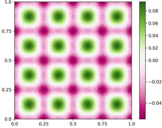
Figure 3: Histogram of particle positions from molecular dynamics simulation of Fig. (2), \sigma = 0.15 . We find a regular 4 \times 4 pattern of peaks in the density. Local density varies by \sim 8\% from the mean. The particle positions of Fig. (2) correspond to a minimum in the probability density.
