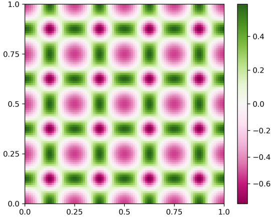
Figure 4: Density variations from a molecular dynamics simulation with 4 particles with \sigma = 0.22 . Positions that are a maximum of density at smaller particle size here become a deep density minimum.
