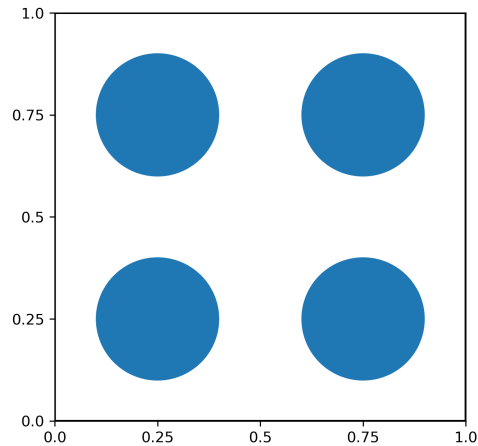
Figure 2: Four particles of radius \sigma = 0.15 are simulated in a square periodic cell with L_x = L_y = 1 .
