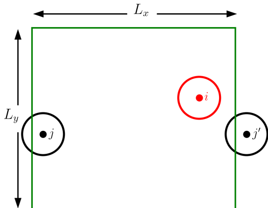
Figure 1: Two particles, i , j have their centers in the periodic cell of volume \Omega = L_x \times L_y . The force between the particles is parallel to the vector joining i and the nearest image of j , j' , eq. (5). The internal virial is calculated between i and j' , requiring a balancing contribution of L_x f_{ij}^x to the second line of eq. (15) which is to be interpreted as a contribution to the momentum flux at the cell edge x = L_x . Here n_x = 1 .
