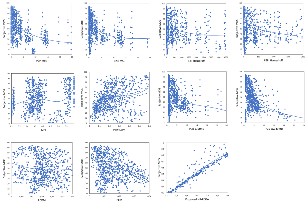
FIGURE 8: Scatter distributions of the objective scores versus the MOS scores on the database WPC. X-axis is the objective quality values predicted by the metrics, Y-axis is the subjective quality scores and the curve presents the estimated no-linear logistic function.
