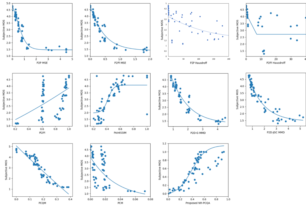
FIGURE 7: Scatter distributions of the objective scores versus the MOS scores on the database SJTU. X-axis is the objective quality values predicted by the metrics, Y-axis is the subjective quality scores and the curve presents the estimated no-linear logistic function.
