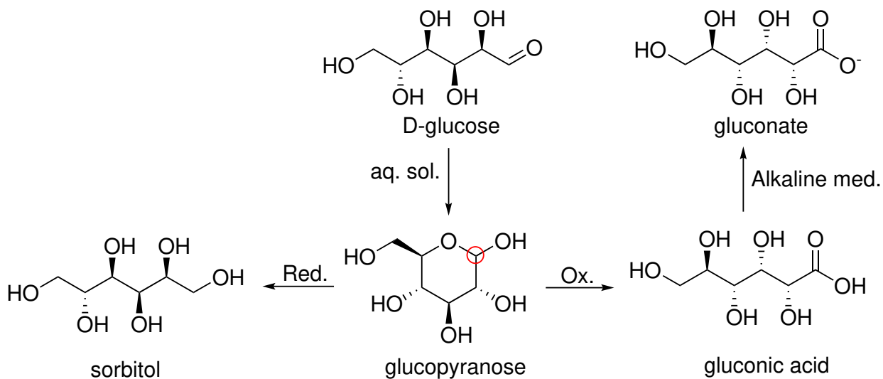
Fig. 1: The simple (electro)chemical reactions of glucose into value-added compounds. In aqueous solution, glucose is mainly under its cyclic form: glucopyranose, that presents an anomeric carbon (circled in red).
