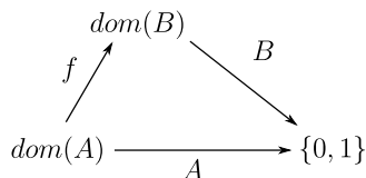
■ Figure 5 The diagram of a many one-reduction, A \preceq_m B when f is computable and the diagram commutes.
