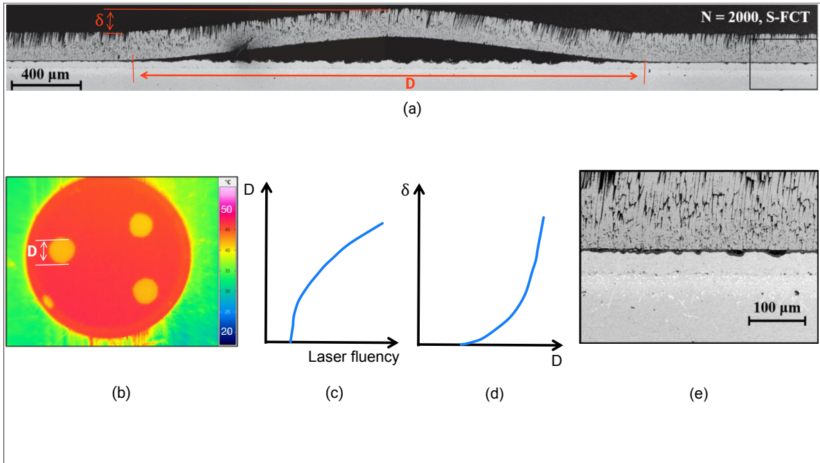
Figure 1: TBC system for LASAT specimen exposed to thermal cycling from 100 to 1100 °C using S-FCT (a) SEM cross-section (b) temperature field on ceramic side after 3 shocks processed by LASAT (c) sketch of the debonded diameter evolution with respect to the laser fluency for LASAT, (d) sketch of the blister height evolution with respect to the debonded diameter and (e) SEM detail of the microstructure far away from the location of the LASAT debonding.
