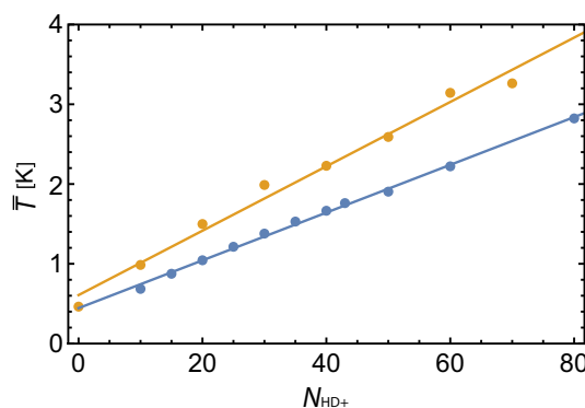
Fig. 19 Results from MD simulations showing the effective Be + ion temperature during a secular scan \bar{T} versus the number of HD + ions N_{\text{HD}^+} , assuming numbers of H 2 D + and HD 2 + ions as in scenario a (blue dots) and scenario b (yellow dots). The blue and yellow lines represent least-squares fits, revealing a linear relationship between \bar{T} and N_{\text{HD}^+}
