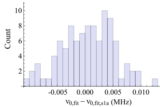
Fig. 16 Histogram of 100 fitted frequencies of the (0, 2)→(8, 3) transition, obtained from a Monte Carlo simulation involving 100 data sets with added random frequency noise (with the noise level corresponding to the measured noise level; see text). On the horizontal axis, zero corresponds to \nu_{0,\text{fit}} obtained for scenario 1a. The mean offset and standard deviation are 0.5 and 8 kHz, respectively
