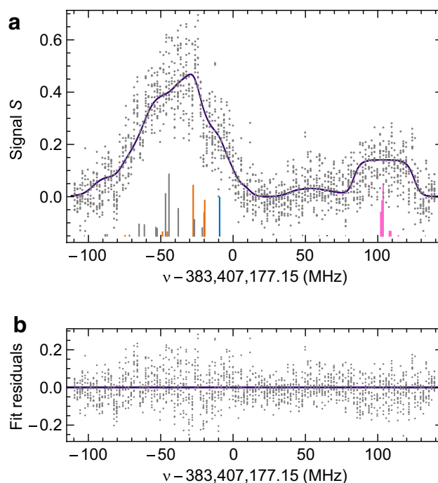
Fig. 14 a Measured spectrum ( dots ) of the (v, L):(0, 2) \rightarrow (8, 3) transition and a least-squares fit ( solid curve ). All 1772 data points are plotted together with the fit function corresponding to scenario 1a. The fitted functions corresponding to the different scenarios are visually indistinguishable from the result shown here. The colored sticks represent the positions and linestrengths of the theoretical individual hyperfine components and are plotted using the same color coding as used in Fig. 2b. b Fit residuals
