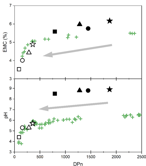
318 Figure 5. Equilibrium moisture content (measured at 30 °C for 50 % RH) and pH of paper as a function of DP_n (initial values ★, humid air 319 ■, humid nitrogen ●, dry air ▲; empty symbols for Whatman paper and full symbols for permanent paper). Literature data for acidic and 320 neutral cotton paper are superimposed (in green crosses, data from [Tétreault et al., 2019]). The progress of ageing is indicated by the arrows.
