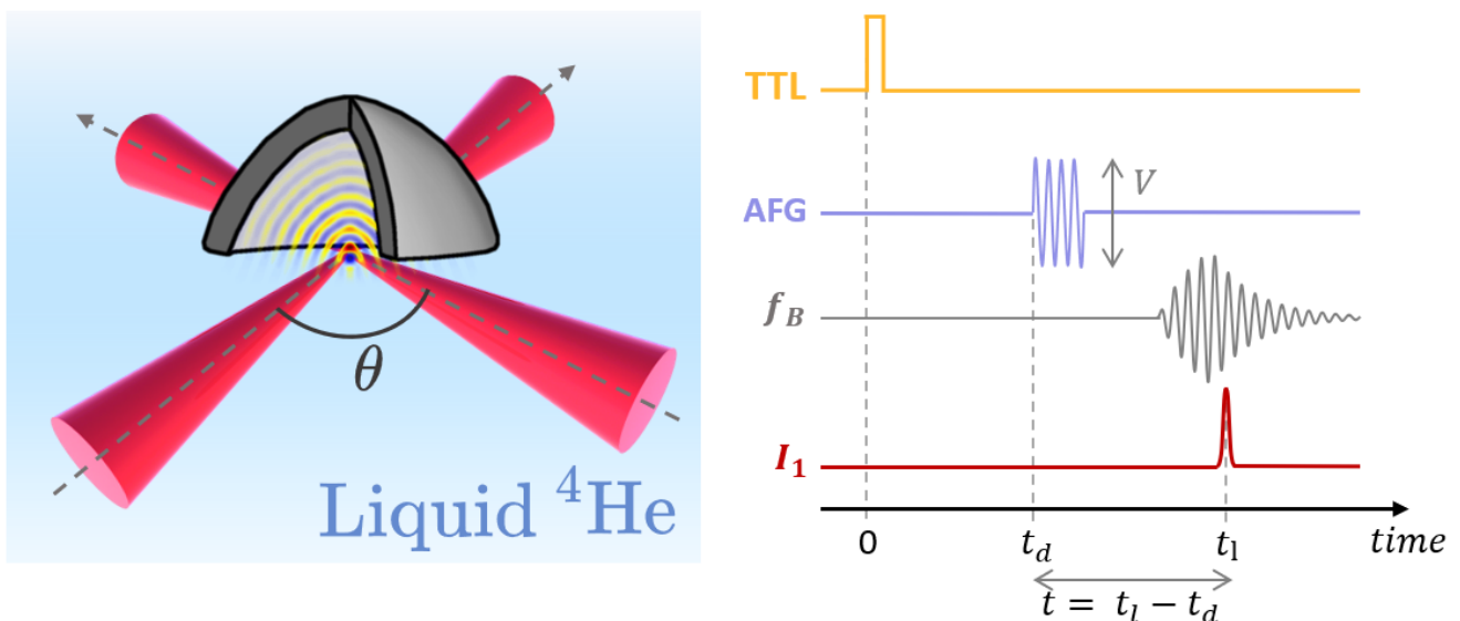
Figure 1: Left: scheme of the experiment. A piezoelectric transducer focuses 1.14 MHz acoustic waves into bulk liquid helium ( T \sim 1 K) producing metastable states during the negative swings of the wave. A SB gain spectrometer consisting of two crossed laser beams, a pulsed pump and a frequency tuneable CW probe, is used to measure time-resolved Brillouin frequencies of the liquid at acoustic focus. \theta is the crossing angle between the lasers. Right: timeline of the experiment. Orange: 10 Hz TTL clock signal delivered by the SB pulsed pump laser, Blue: driving piezo transducer voltage (amplitude V , frequency f_{ac} ), Gray: Brillouin frequency at acoustic focus, Red: Pump SB laser intensity I_1 .
