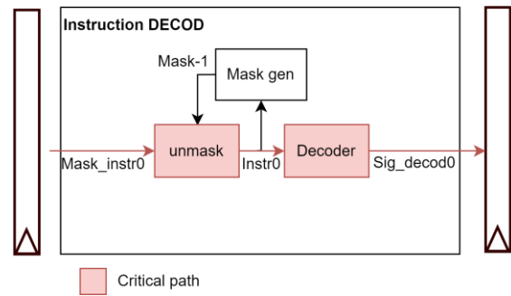
Figure 1: Signals Pre-Decoder
