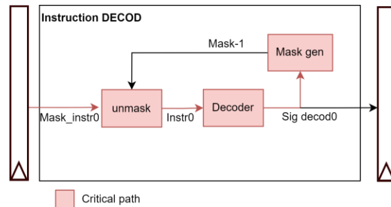
Figure 2: Signals Post-Decoder
