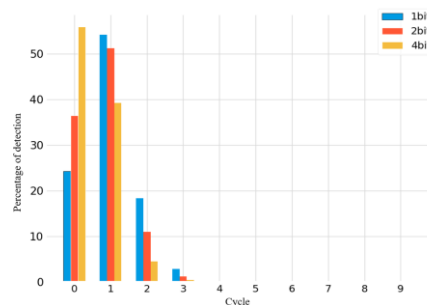
Figure 13: Multiple fault
