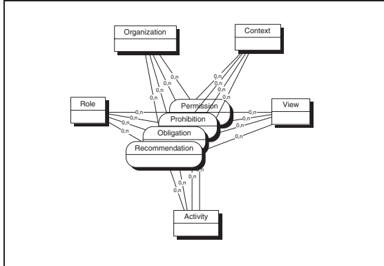
Figure 5: The Permission , Prohibition , Obligation and Recommendation relationships
