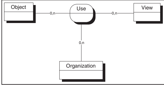
Figure 2: The Use relationship
