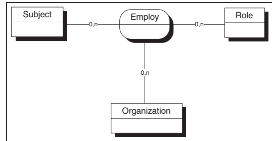
Figure 1: The Employ relationship
