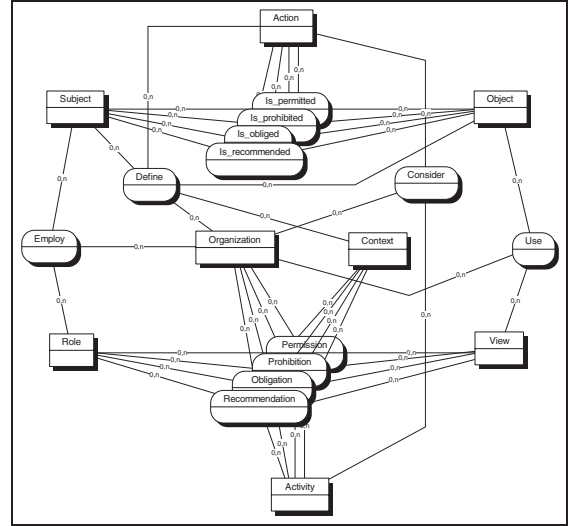
Figure 6: The ORBAC model
