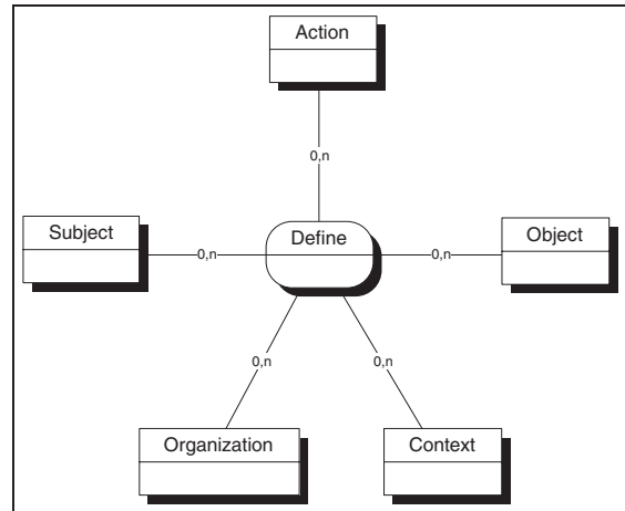
Figure 4: The Define relationship
