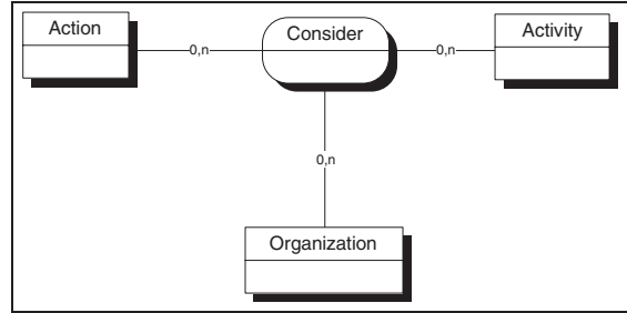
Figure 3: The Consider relationship
