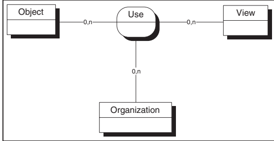
Figure 2: The Use relationship
