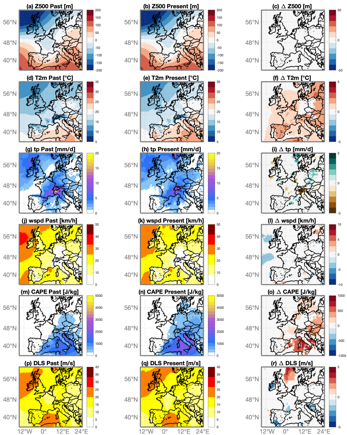
Figure 5. Attribution for the 18 August 2022 derecho storm. Average of the 37 analogues of daily mean zero-centred geopotential height anomaly at 500 hPa (Z500) found for the counterfactual (1950–1980) (a) and factual (1992–2022) (b) periods and corresponding 2 m temperatures (T2m) (d, e), daily total precipitation (tp) (g, h) and wind speed (wspd) (j, k). Changes in the corresponding variables: \Delta Z500 (c), \Delta T2m (f), \Delta tp (i) and \Delta wspd (l) between factual and counterfactual periods (coloured-filled areas show significant anomalies with respect to the bootstrap procedure).
