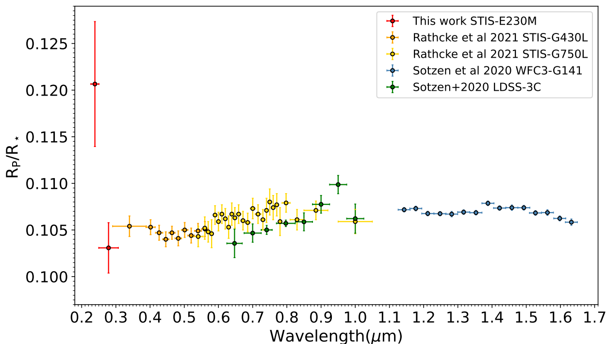
Fig. 4. WASP-79b HST transmission spectrum. NUV values are from the broadband analysis of visit #66 obtained here using the STIS E230M observations (in red). For clarity, we represent two values around 2400Å and 2700Å (Bins 1 and 2 in Table 6). The optical values are from the analysis of Rathcke et al. (2021) of STIS G430L and G750L data (orange and yellow). HST WFC3 observations in the NIR are from Sotzen et al. (2020) (blue).
