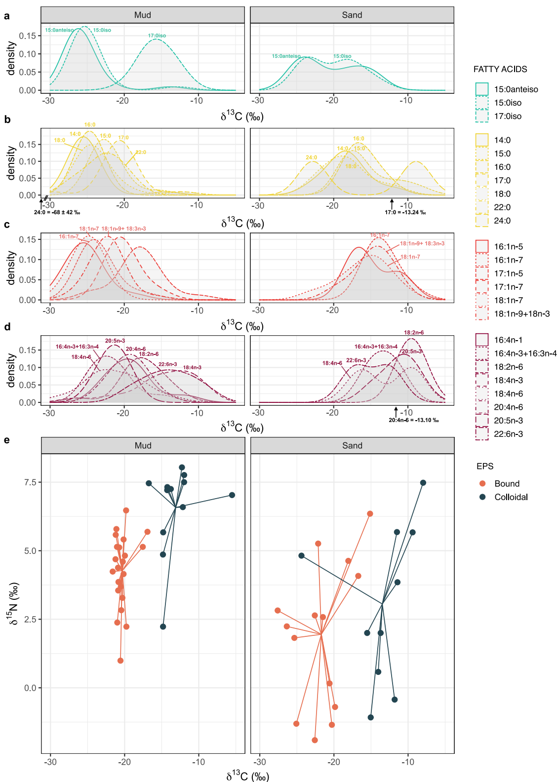
Figure 4 – C and N isotopic ratio of fatty acids and EPS fractions. a-d : Kernel density estimates of \delta^{13}C of fatty acid biomarkers (corrected according to equation 1). e : \delta^{13}C and \delta^{15}N biplots of bound and colloidal EPS. All sampling points were grouped together. In panels a-d , fatty acids are grouped by classes they belong to according to fig.3
