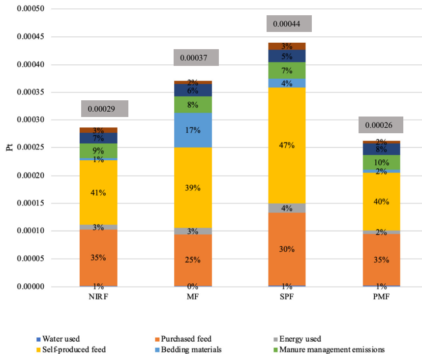
Fig. 4. Process contribution to the total score for each farm system considered.
