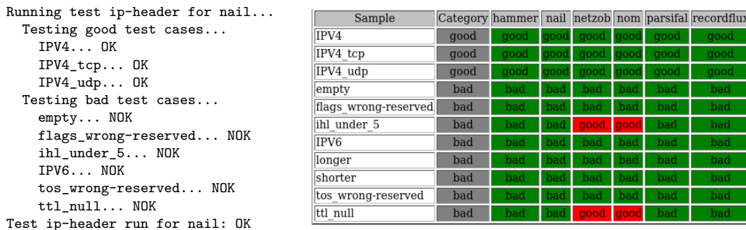
Figure 2: Execution of Nail implementation for the IP Header (on the left). Results for various IP Header parsers against the samples (on the right).
