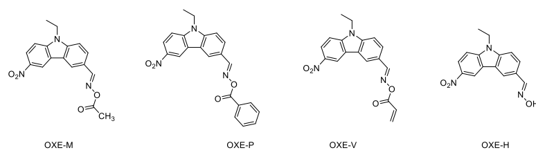
Scheme 6. Chemical structures of the nitrocarbazole-based oxime esters OXE-M , OXE-V , OXE-P and OXE-H .
