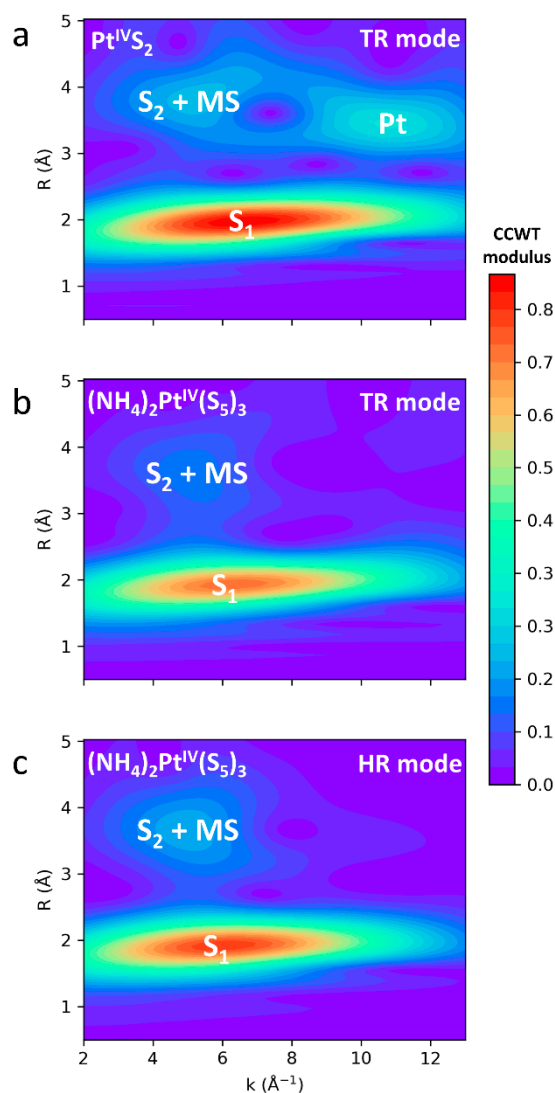
Figure 8. Wavelet analysis of k^2 -weighted EXAFS spectra of \text{Pt}^{\text{IV}}\text{S}_2 -s (a) and (\text{NH}_4)_2\text{Pt}^{\text{IV}}(\text{S}_5)_3 in TR mode (b) and HR mode (c), with the CCWT modulus showing the (k, R) localization of each EXAFS contribution ( S_1 = 1\text{st Pt shell} , S_2 = 2\text{nd Pt shell} , \text{MS} = \text{multiple scattering arising from the 1st Pt shell} ). No contributions from atoms heavier than S appear in (\text{NH}_4)_2\text{Pt}^{\text{IV}}(\text{S}_5)_3 , either in TR or HR mode, in contrast with \text{Pt}^{\text{IV}}\text{S}_2 -s showing strong contributions from the heavy Pt atoms in the 2nd shell.
