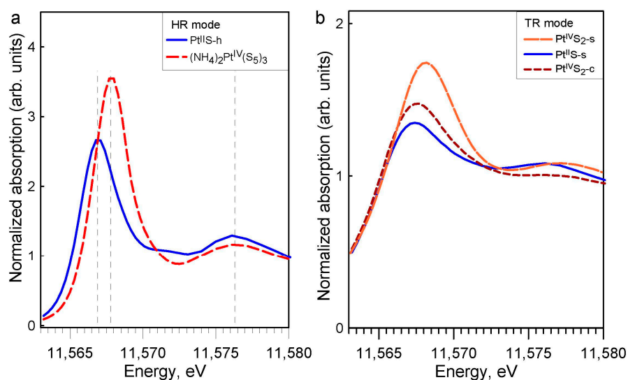
Figure A3. (a) Normalized Pt L_{\text{III}} -edge XANES spectra in HR mode for the two Pt-S solid compounds, \text{Pt}^{\text{II}}\text{S-h} and (\text{NH}_4)_2\text{Pt}^{\text{IV}}(\text{S}_5)_3 . (b) Normalized Pt L_{\text{III}} -edge XANES spectra in TR mode for synthesized \text{Pt}^{\text{II}}\text{S-s} , \text{Pt}^{\text{IV}}\text{S}_2\text{-s} , and \text{Pt}^{\text{IV}}\text{S}_2\text{-c} . The commercial \text{Pt}^{\text{IV}}\text{S}_2\text{-c} solid is impure, containing mostly PtS and S with a little amount of \text{PtS}_2 .
