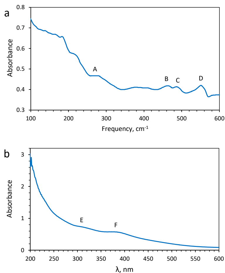
Figure A2. (a) Far-infrared spectrum and (b) UV-visible spectrum of synthesized (\text{NH}_4)_2\text{Pt}^{\text{IV}}(\text{S}_5)_3 . The main absorbance peaks in (a) are at 278 \text{ cm}^{-1} (A), 461 \text{ cm}^{-1} (B), 487 \text{ cm}^{-1} (C), 551 \text{ cm}^{-1} (D). The two main absorbance peaks above the cutoff of 200 nm in (b) are at 290 nm (E) and 385 nm (F).
