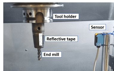
(b) Sensor setup
