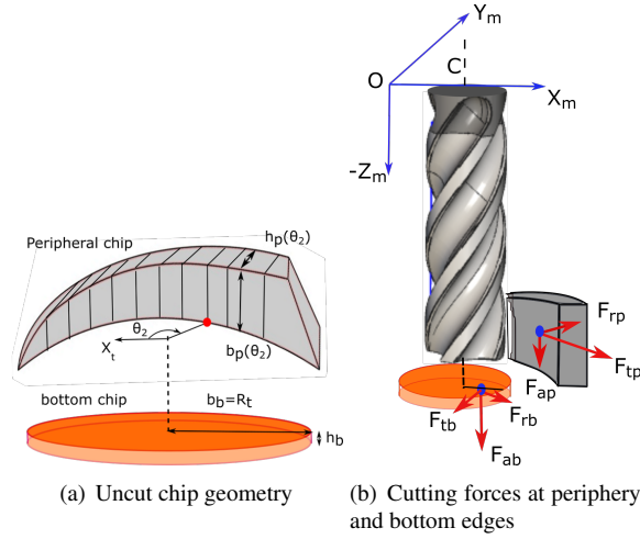
Figure 2: Chip generation and cutting forces during helical milling
