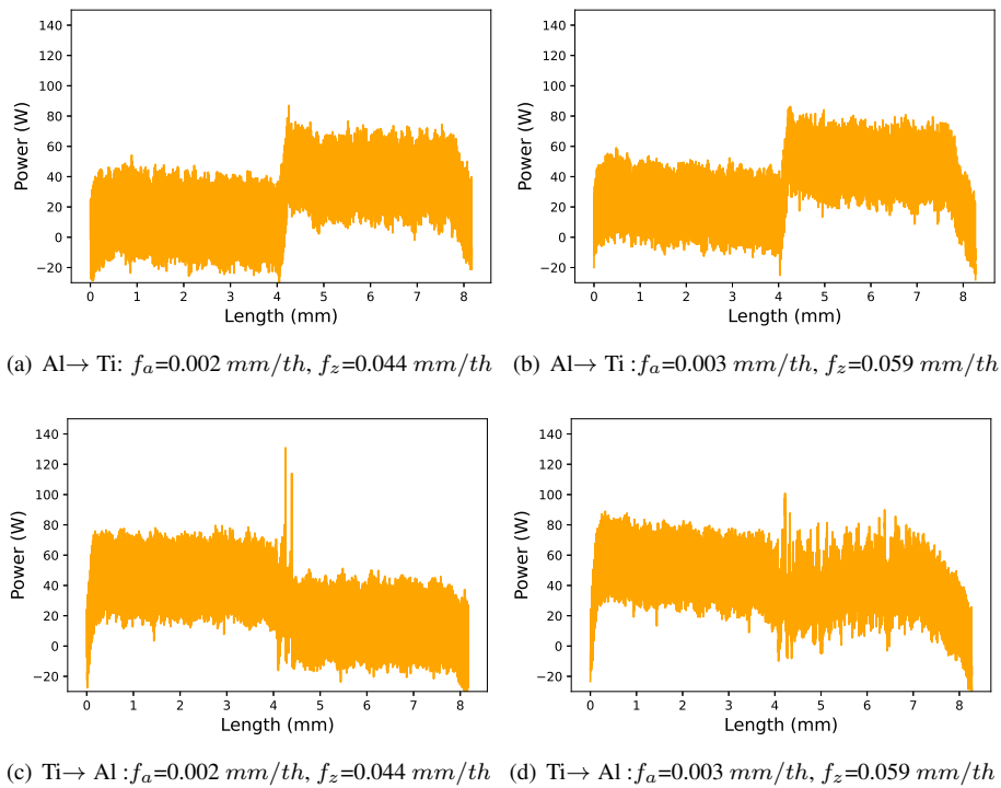
Figure 7: Spindle power as a function of hole depth at different cutting conditions.
