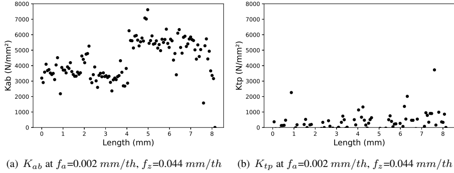
Figure 9: Data map of cutting force coefficients for Al→ Ti stack
