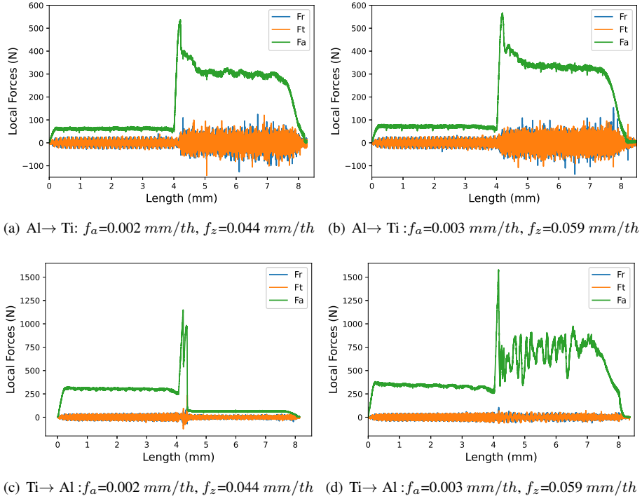
Figure 8: Local cutting forces as a function of hole depth at different cutting conditions.
