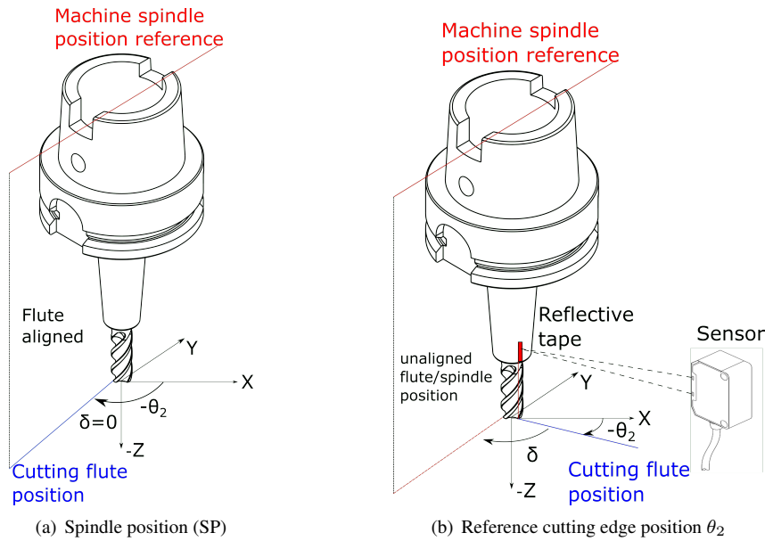
Figure 5: Identification of reference flute position
