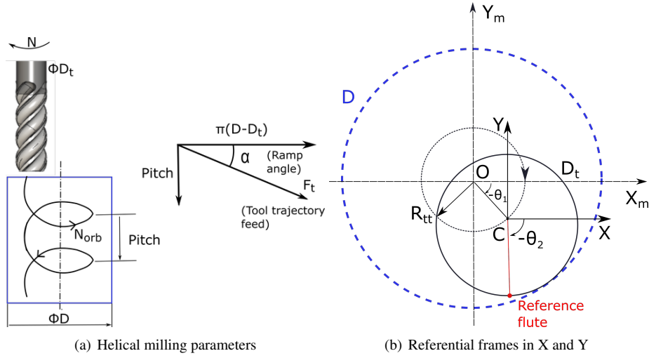
Figure 1: Tool trajectory in orbital drilling
