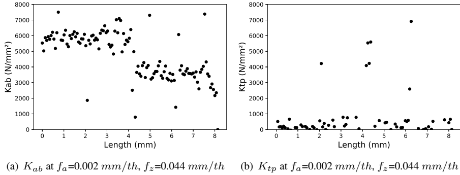
Figure 10: Data map of cutting force coefficients for Ti→ Al stack
