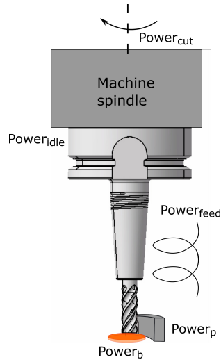
Figure 3: Spindle power components
