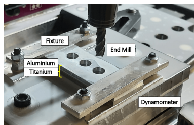
(a) Al/Ti stack
