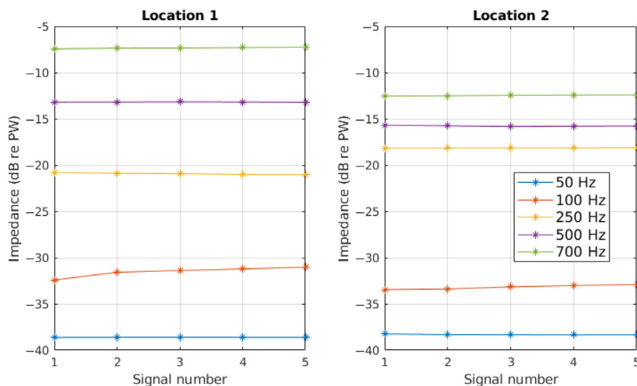
Fig. 5. Acoustic impedance as measured at two different positions in the tank. Note that the impedance is given in dB relative to Plane Wave propagation, that is, 0 dB means that PE = KE, as is the case for a plane wave.
