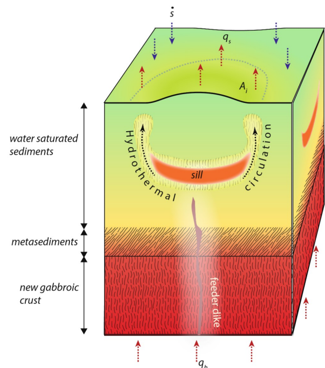
FIGURE 8 Representative volume of the Guaymas Basin, central Gulf of California. The elements contained in the control volume govern the thermal evolution of the basin at different time scales according to the balance of heat discussed in the main text. q_b is the basal (background) heat flow; q_s is the superficial heat flow; s represents the rate at which new mass enters the reference volume; A_i is the area of the sill.
