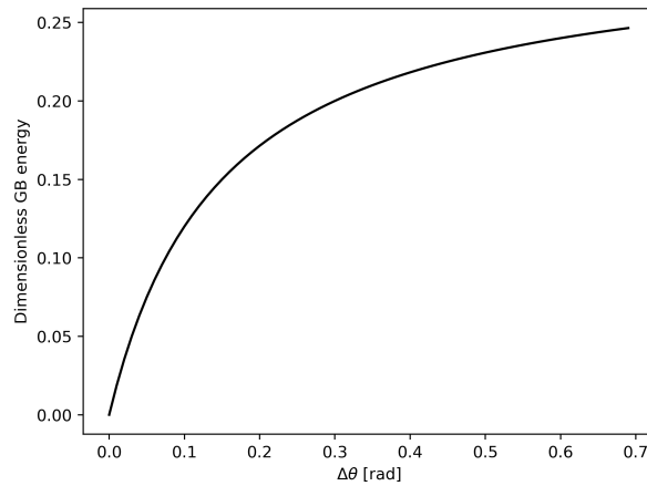
Fig. 4 Dimensionless grain boundary energy-misorientation curve
