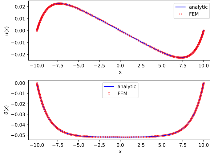
Fig. 2 Cosserat elasticity, displacement and microrotation fields. Finite Element simulations are compared to the analytical solution, based on the material parameters of table 1.
