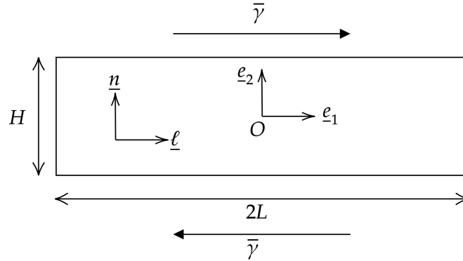
Fig. 1 Geometry of the simple shear boundary value problem in crystal plasticity involving a single slip system.
