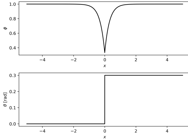
Fig. 3 Profiles of \phi and \theta in the sharp interface case
