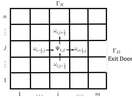
FIGURE 1. Discretization of the domain \Omega .
