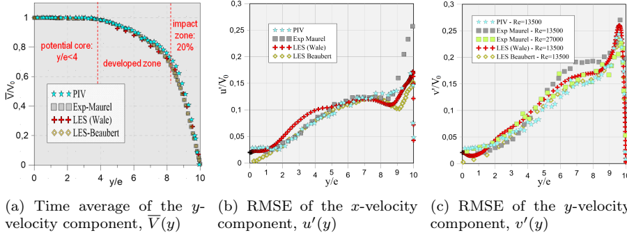
Fig. 4: Profiles of the time averages and RMSE of the x - and y -velocity components along the jet y -axis, at Re_j \approx 13500 unless otherwise stated.
