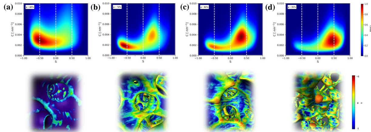
Figure 11. Pore curvature maps for 3D reconstructed alumina Al 1.3 \mu m (in Figure 3) at (a) the initial stage and after sintering at 1500°C and observing post-mortem at (b) 1 hour, (c) 10 hours and (d) 30 hours respectively, along with snapshots of cropped sections of the 3D rendering of the pore network.
