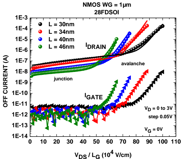
Figure 15: I_{DS} and I_G measurements and modeling at T=125^\circ\text{C} under Off-state ( V_{GS}=0 ) for L_G=30\text{nm} to 46\text{nm} NFETs as a function of peak lateral field approximated to E_{max} \approx V_{DS} / L_G showing a junction leakage and avalanche components in the diode currents. The modeling is shown in lines for I_{DS} monitoring with relatively good agreements as a function of gate-length L_G .
