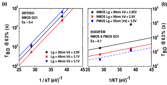
Figure 11: Temperature dependence of T_{BD} (63%) under Off-state stressing (a) in 28FDSOI NFEETs and (b) in 65SOI P- and N- FETs extracted from 125 °C to 25 °C. The activation energy ( E_a ) remains constant for different gate channel length.
