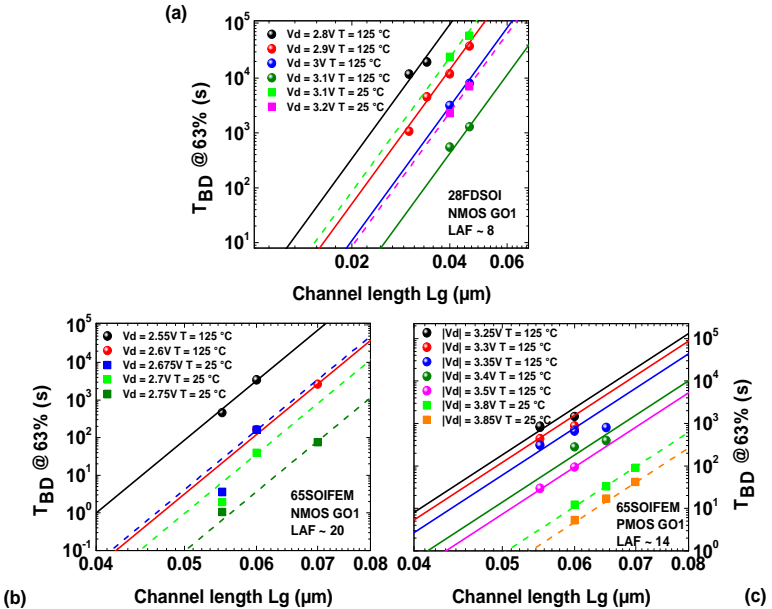
Figure 10: TDDB in GO1 28FD and 65FEM obtained at 63% vs. channel length L_G with various drain voltage (reverse case of Fig. 8 ) in order to extract acceleration factors LAF at 125°C (solid lines) and 25°C (dashed lines). (a) 28nm NFETs, (b) 65nm NFETs and (c) 65nm PFETs. A common LAF is extracted independently of drain bias and temperature.
