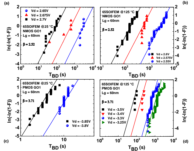
Figure 6: Weibull distribution plots for GO1 W_G/L_G = 10\mu\text{m}/60\text{nm} 65 SOI NFET and PFET at various drain voltage (a) NFET at 25 °C, (b) NFET at 125 °C, (c) PFET at 25 °C and (d) PFET at 125 °C. Weibull distribution slopes \beta are higher in PMOS than in NMOS an independent of bias&temperature.
