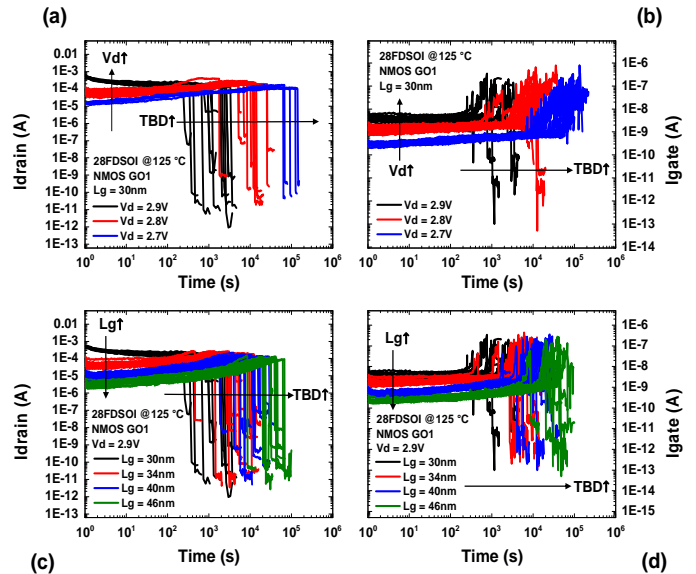
Figure 1: Leakage current until breakdown in 28nm FDSOI NFETs W_G = 1\mu\text{m} with various V_{DS} and L_G as a function of cumulative stress time. (a) drain and (b) gate initial currents increasing with V_{DS} for L_G=30\text{nm} . Initial leakage current is smaller for longer devices, (c) drain current and (d) gate current monitors decreasing with L_G at the same bias V_{DS} = 2.9\text{V} .
