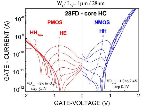
Figure 3: Consequence of Impact Ionization shown in NFET and PFET W_G / L_G = 1\mu\text{m} / 28\text{nm} FDSOI under HC mode seen by gate current ( I_{gate} ) measurements in thin gate-oxide for V_{DS} and V_{GS} variables, showing the distinct injection mechanisms between hot-electrons and hot-holes at low V_{GS} which turns around to a single tunneling component at high V_{GS} .
