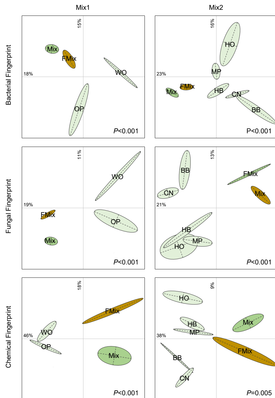
Figure 3. Differences in bacterial, fungal and chemical composition of the two mixtures of forest litters. Mix1 (WO: white oak, OP: holm oak and Aleppo pine) and Mix2 (BB: bamboo, CN: chestnut, HB: hackberry, HO: holm oak, MP: maritime pine). Mix: mixture of litters before fermentation, FMix: mixture of litters after fermentation). Between Class Analysis (BCA) is based on bacterial
