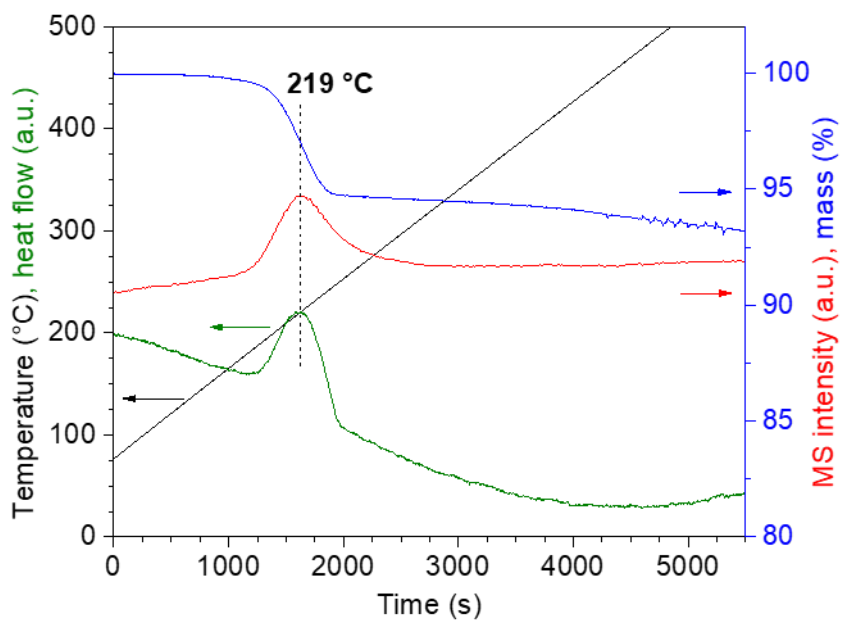
Figure 6. Evolution of mass (%), temperature (°C) and heat flow (a.u.) during TGA ( 5\text{ }^{\circ}\text{C min}^{-1} ) under 3% v/v \text{H}_2/\text{Ar} and associated \text{H}_2\text{O} MS signal ( m/z = 18 ) for 21Cu-SI.
