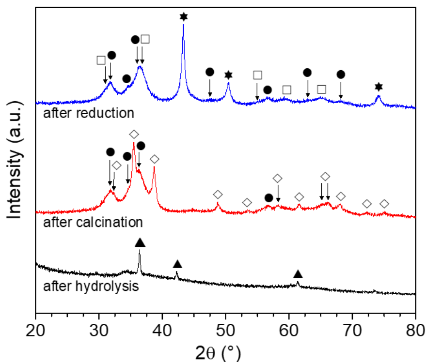
Figure 2. XRD diffractograms associated with 25Cu-16Al-S1 i) after hydrolysis, ii) after calcination at 400 °C and iii) reduction at 350 °C and passivation. Symbols refer to peaks associated with (▲) Cu 2 O (Pn-3m, PDF 00-005-0667), (●) ZnO (P63mc, PDF 01-079-0205), (◇) CuO structure (C2/c, PDF 00-045-0937), (□) ZnAl 2 O 4 (Fd-3m, PDF 04-014-1594) and (★) Cu (Fm-3m, PDF 04-13-9963).
