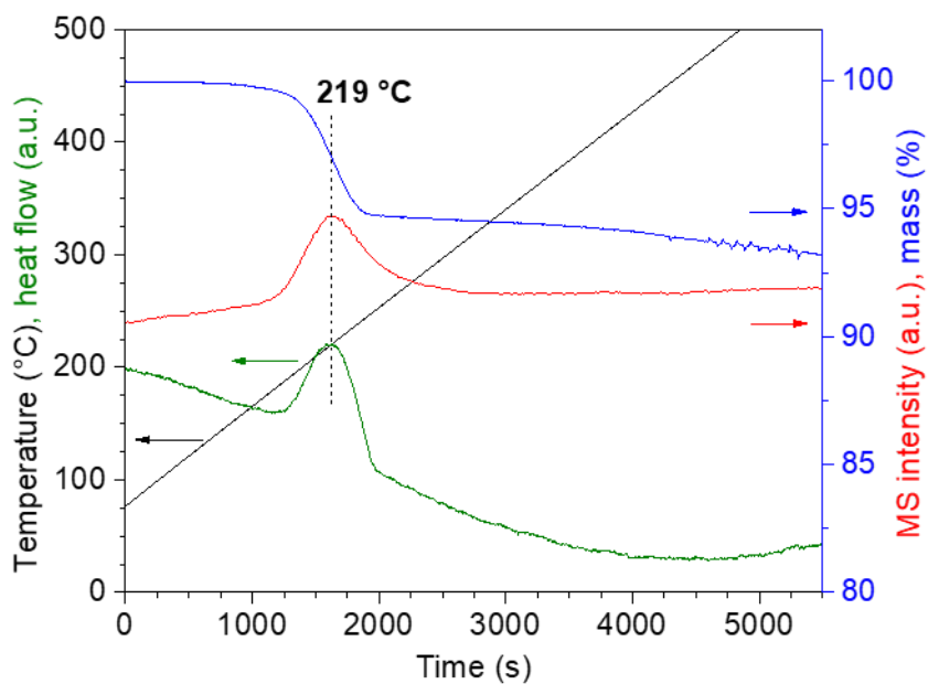
Figure 6. Evolution of mass (%), temperature (°C) and heat flow (a.u.) during TGA ( 5\text{ °C min}^{-1} ) under 3% v/v H_2/Ar and associated H_2O MS signal ( m/z = 18 ) for 21Cu-SI.
