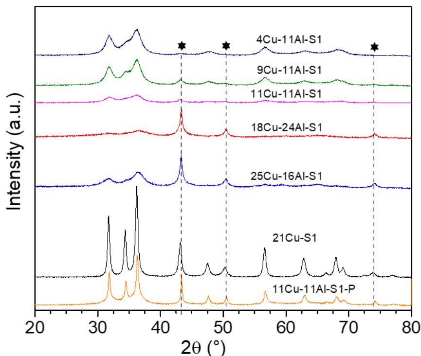
Figure 3. XRD diffractograms associated with 4Cu-11Al-S1, 9Cu-11Al-S1, 11Cu-11Al-S1, 18Cu-24Al-S1, 25Cu-16Al-S1, 21Cu-S1 and 11Cu-11Al-S1-P. Symbols (★) refer to Cu ( Fm\text{-}3m , PDF 04-13-9963). The other peaks are associated with ZnO and \text{ZnAl}_2\text{O}_4 .
