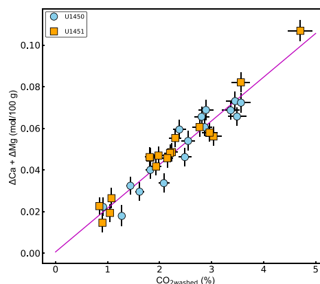
Figure F9. Comparison between CO 2 measured in washed sediments and sum of leached Ca and Mg ( \Delta\text{Ca} + \Delta\text{Mg} ), Sites U1450 and U1451. Error bars = analytical uncertainties. Purple line = error weighted regression line ( y = \{0.021 \pm 0.001\}x + \{0 \pm 0.002\} ).
