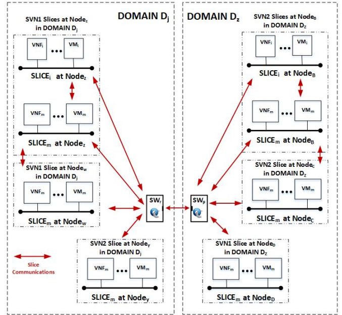
Figure 2. A Generic SVN with Slices View
