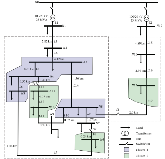
FIGURE 1 Topology of the CIGRE European MV distribution network benchmark for residential system [21].
