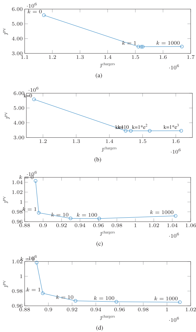
FIGURE 3 Change in PV self-consumption J^{PV} (lower values denote better PV self-consumption) with the cost of the recharging infrastructure J^{chargers} , for increasing values of k in different scenarios: forgetful EV owners (a), Cooperative EV owners (b), forgetful EV owners with extended daytime parking intervals (c), and cooperative EV owners with extended daytime parking intervals (d).
