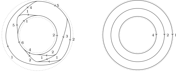
FIGURE 4. Two vinyl graphs of index 7, the one on the right-hand side is \mathbb{S}_{(4,2,1)} .
